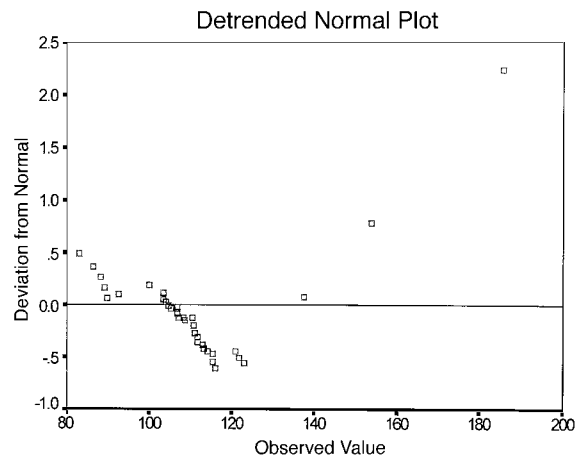
FIG. 7. Normal Probability Plots for Time Variance
