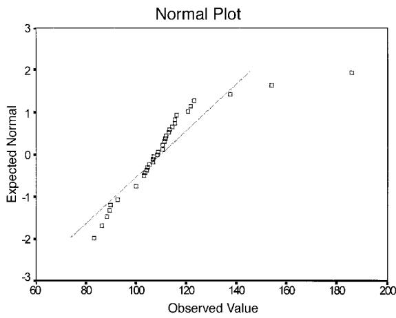
FIG. 7. Normal Probability Plots for Time Variance
